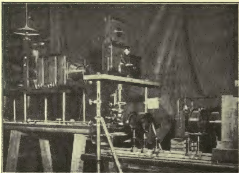
FIG. 39.—V. Henri's apparatus for photographing Brownian movement cinematographically.
